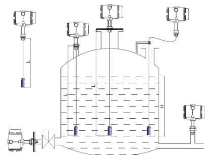
Vessel Installation
